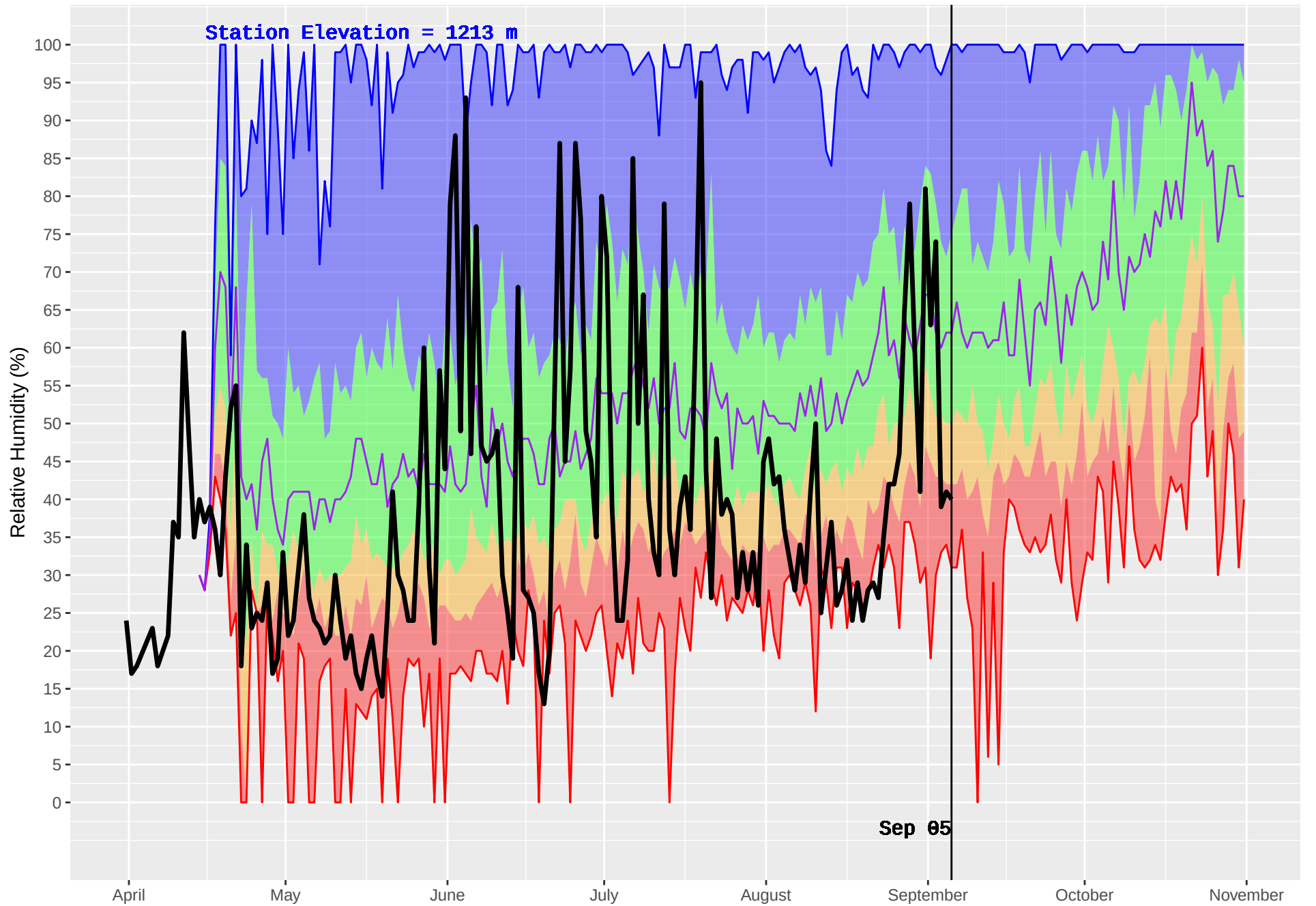
INGENIKA POINT (145) : Historical (1971–2016) and Current (2018) Daily Relative Humidity
